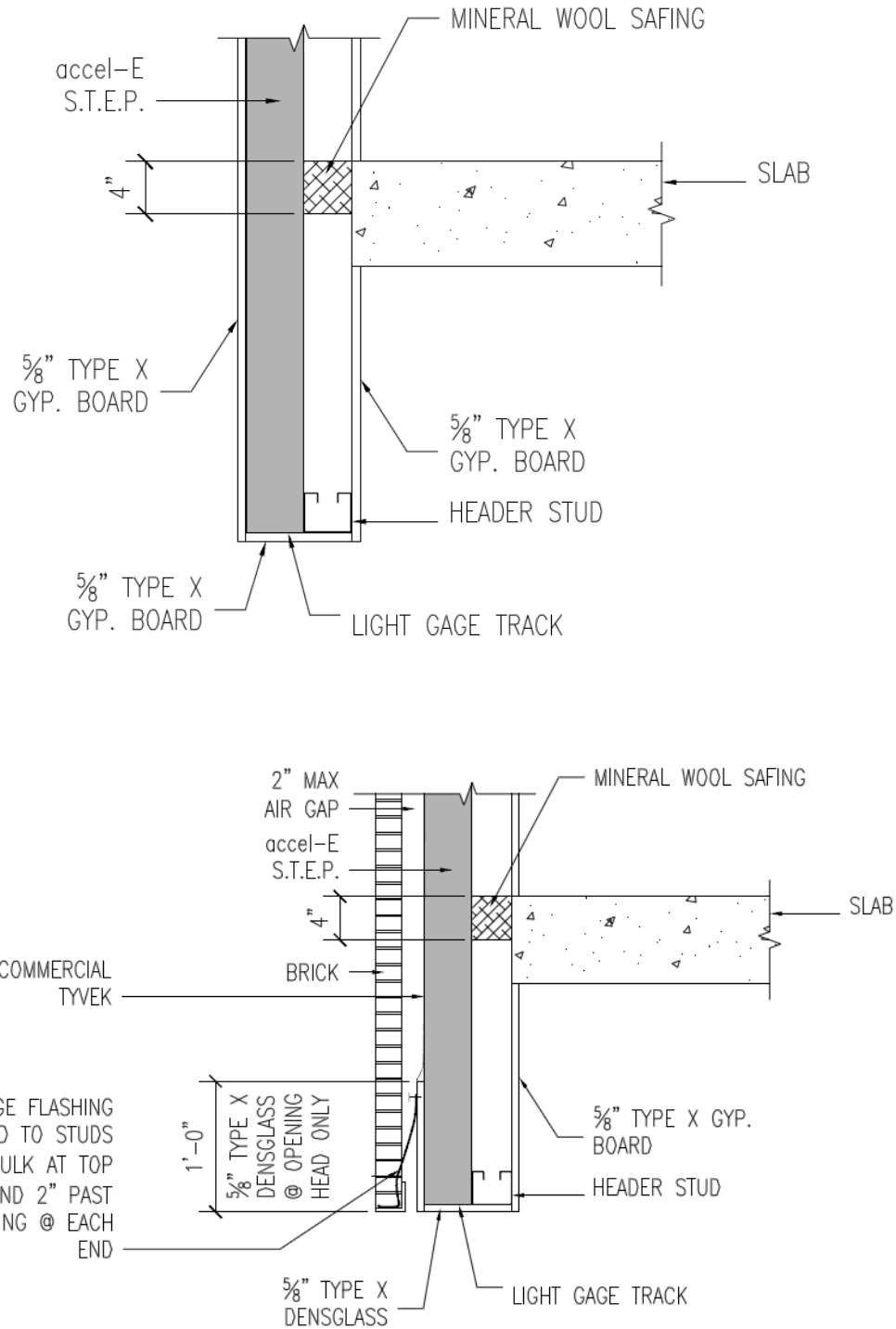
Figure 9 – NFPA 285 Details
